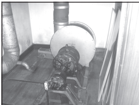
Tschantz Pipe Organ Blower
